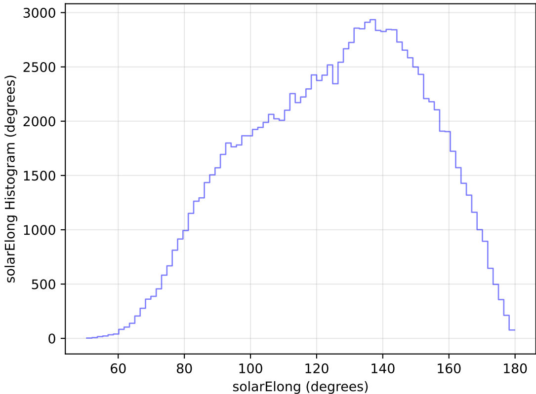
weather_cloudso1v3.4_10yrs WFD u band: solarElong Histogram
