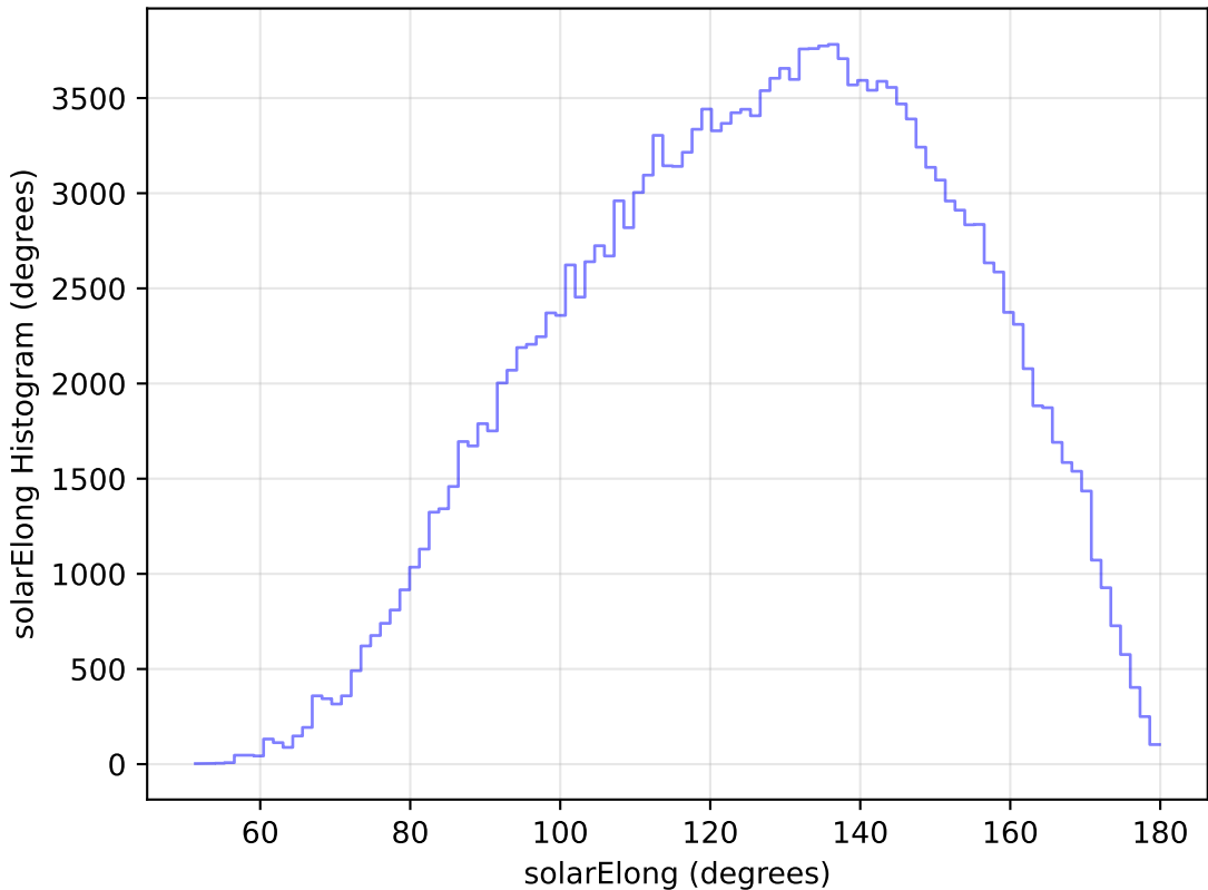
weather_cloudso1v3.4_10yrs WFD g band: solarElong Histogram
