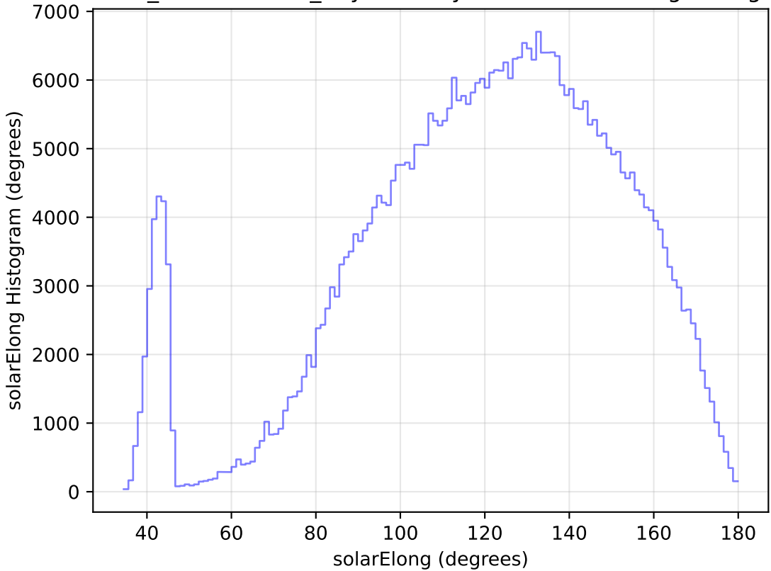
weather_cloudso1v3.4_10yrs All sky z band: solarElong Histogram
