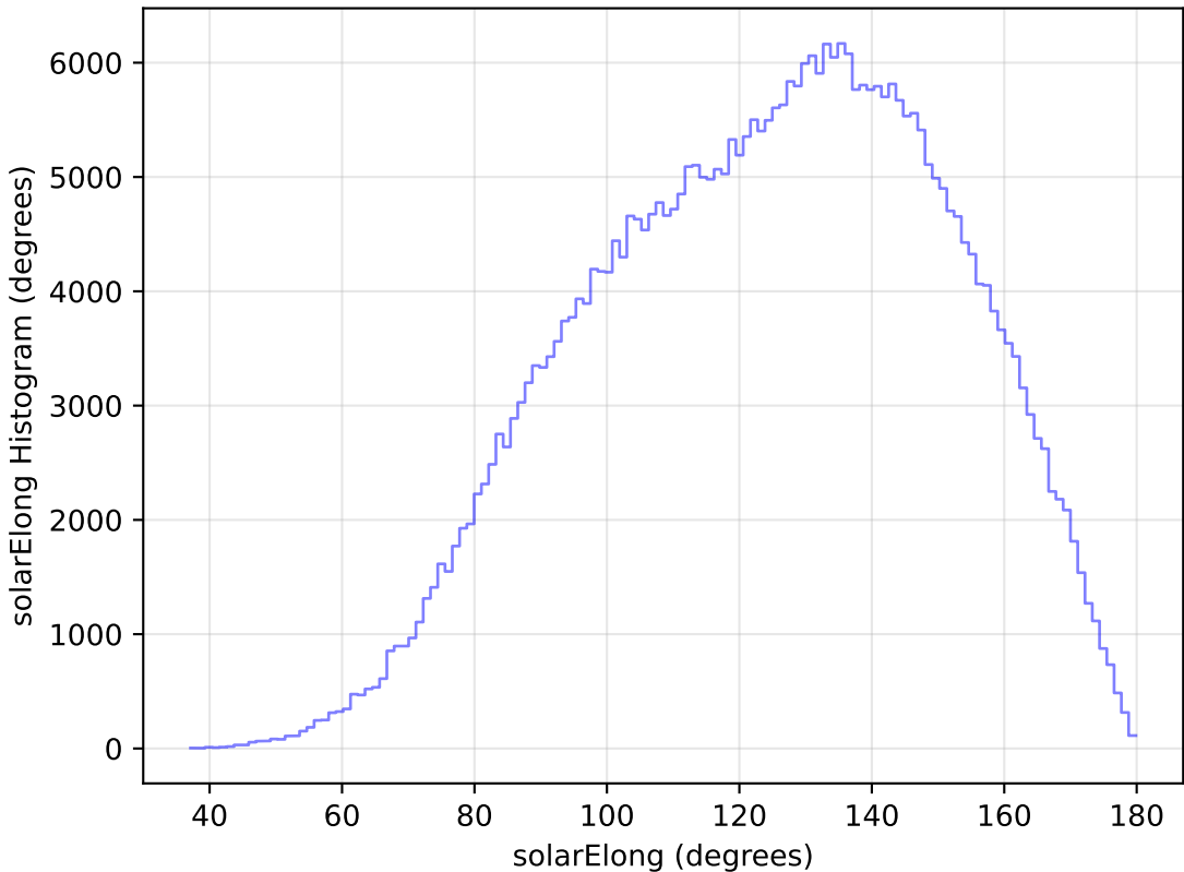
weather_cloudso1v3.4_10yrs All sky y band: solarElong Histogram
