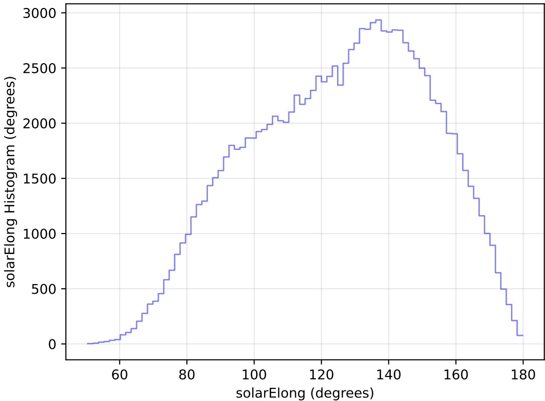
weather_cloudso1v3.4_10yrs All sky u band: solarElong Histogram
