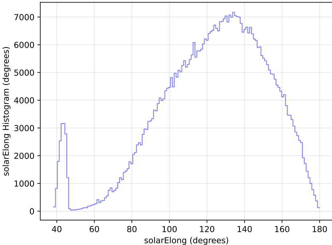
weather_cloudso1v3.4_10yrs All sky r band: solarElong Histogram
