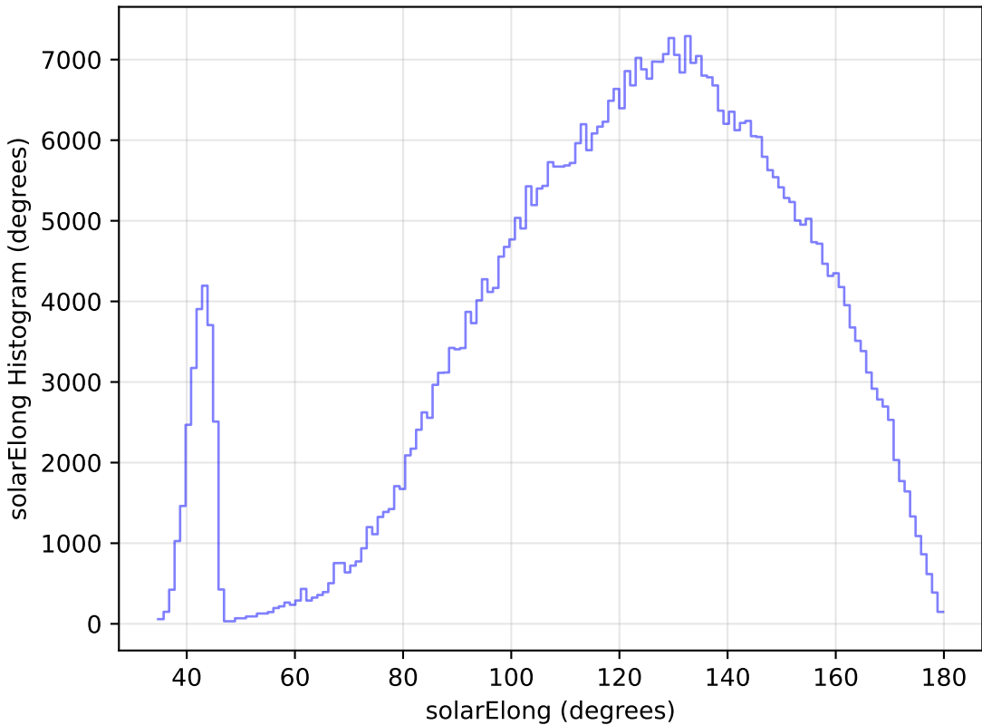
weather_cloudso1v3.4_10yrs All sky i band: solarElong Histogram
