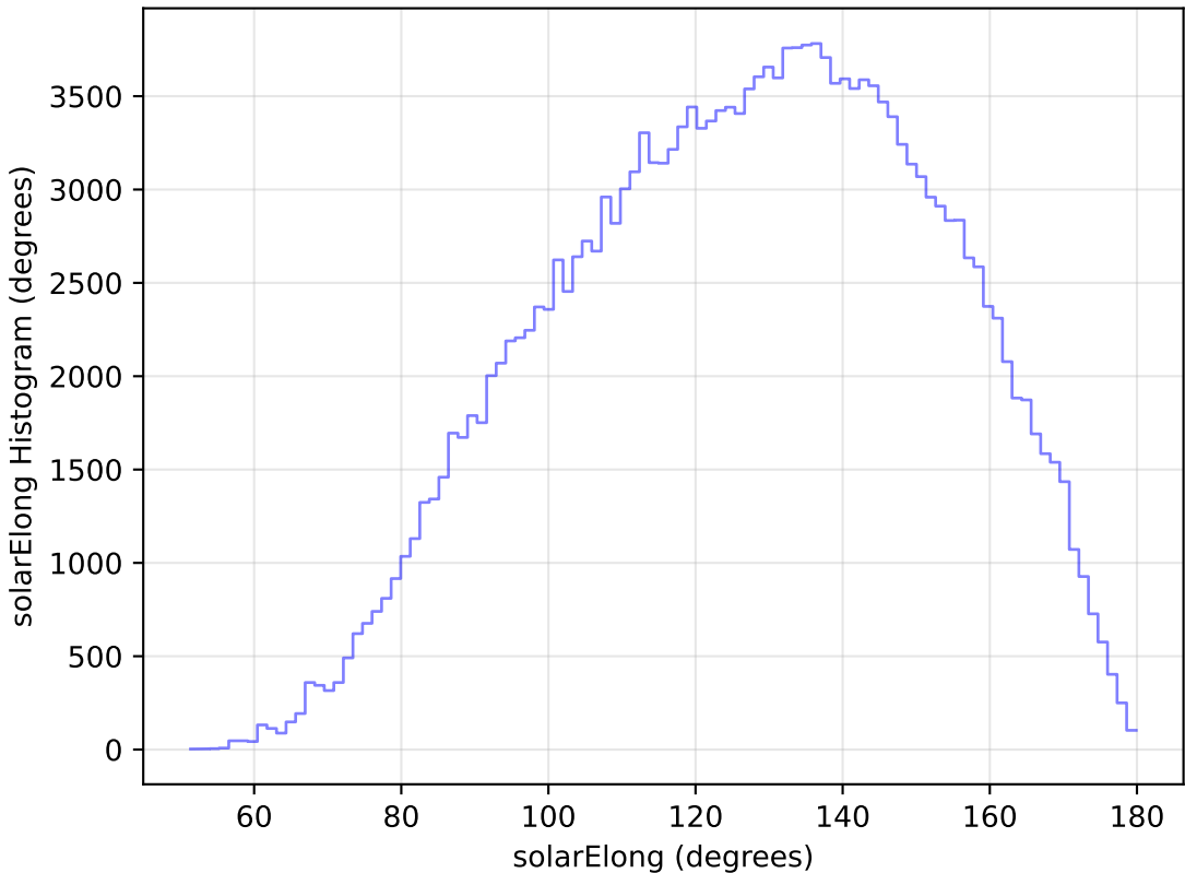
weather_cloudso1v3.4_10yrs All sky g band: solarElong Histogram
