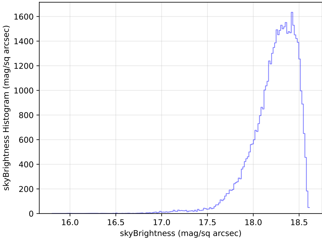
weather_cloudso1v3.4_10yrs Yr 1 y band: skyBrightness Histogram
