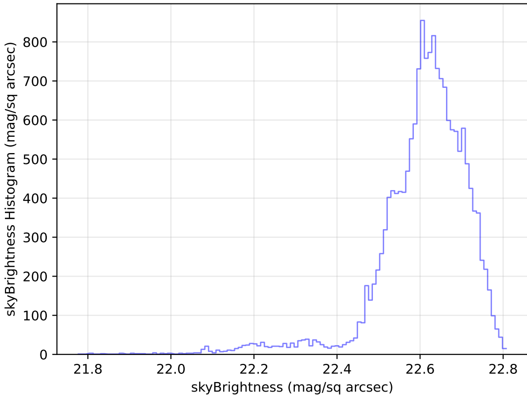
weather_cloudso1v3.4_10yrs Yr 1 u band: skyBrightness Histogram
