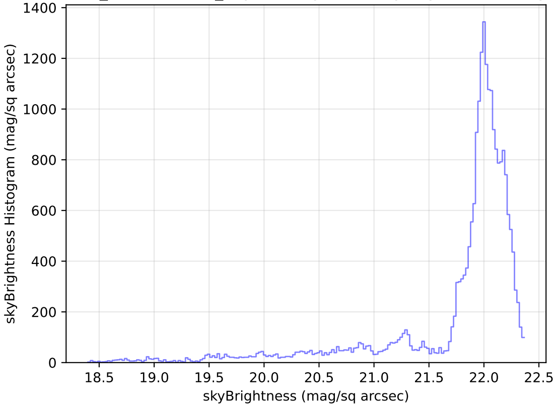
weather_cloudso1v3.4_10yrs Yr 1 g band: skyBrightness Histogram
