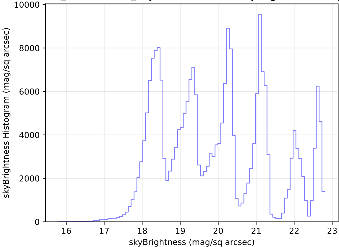
weather_cloudso1v3.4_10yrs Yr 1 all bands: skyBrightness Histogram
