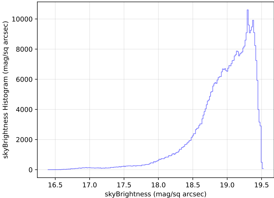
weather_cloudso1v3.4_10yrs WFD z band: skyBrightness Histogram
