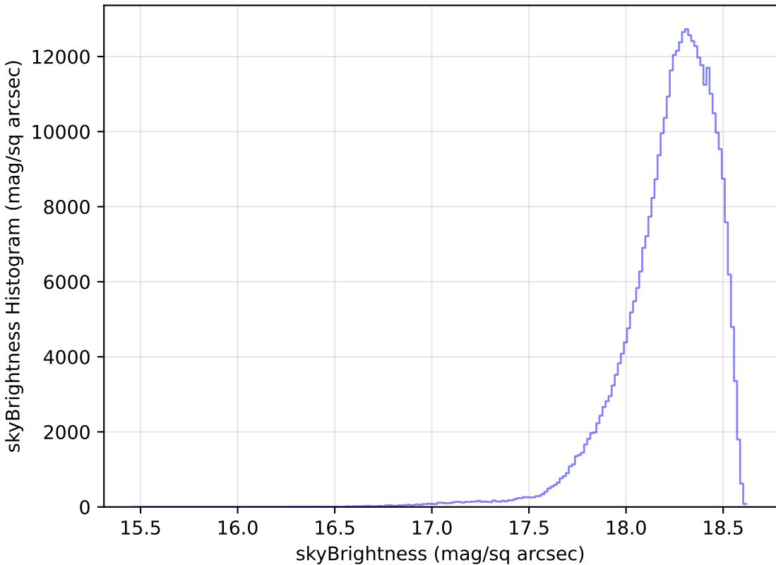
weather_cloudso1v3.4_10yrs WFD y band: skyBrightness Histogram
