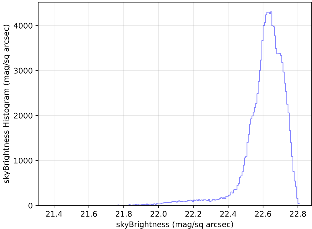
weather_cloudso1v3.4_10yrs WFD u band: skyBrightness Histogram
