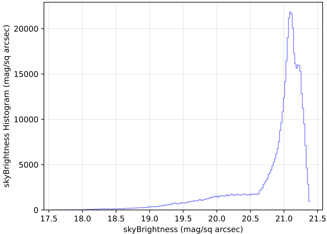
weather_cloudso1v3.4_10yrs WFD r band: skyBrightness Histogram
