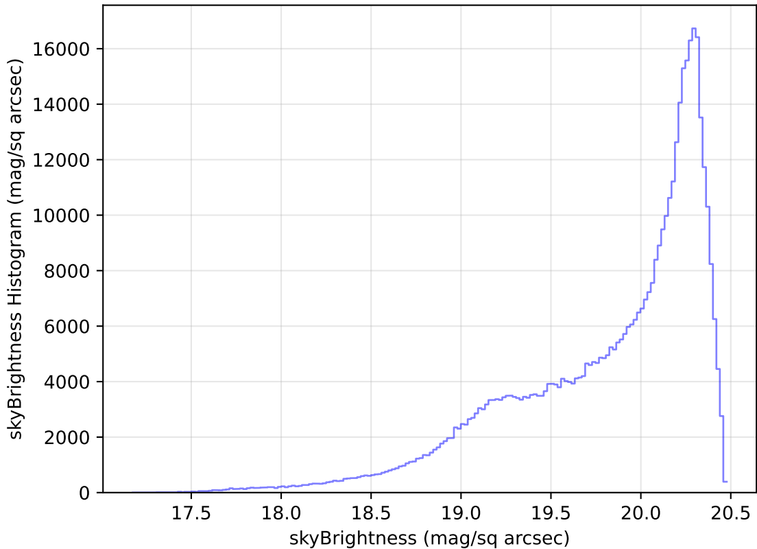
weather_cloudso1v3.4_10yrs WFD i band: skyBrightness Histogram
