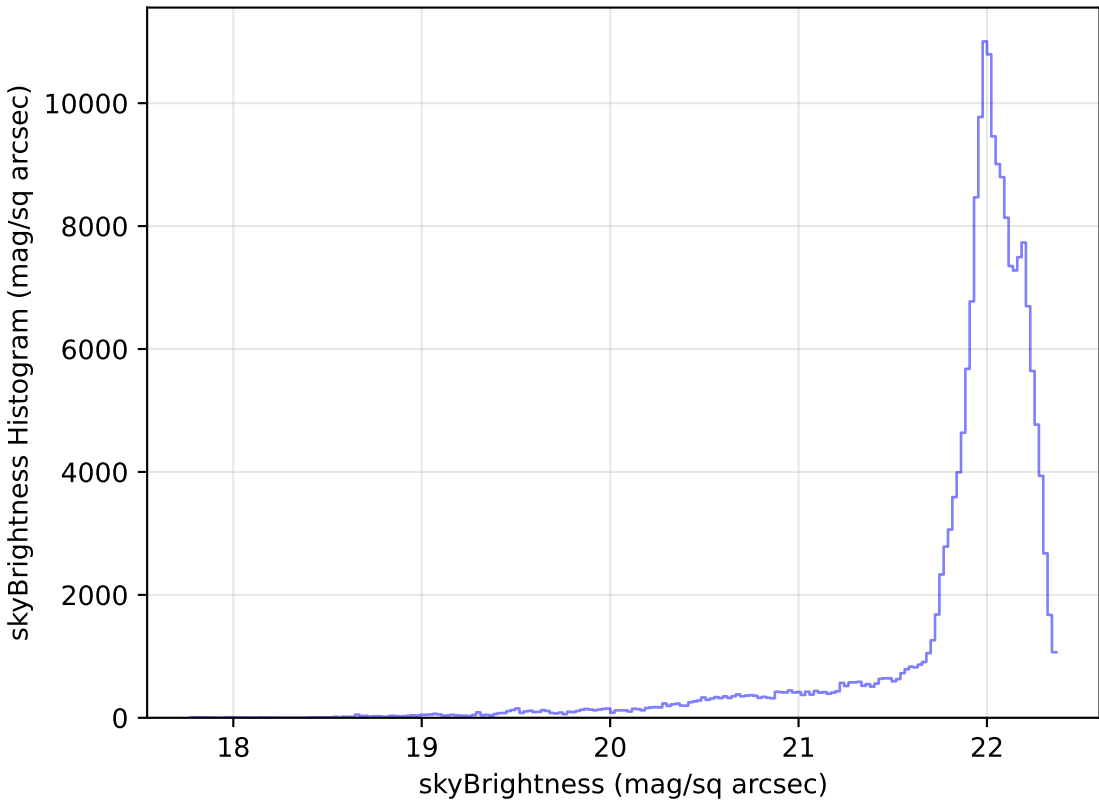
weather_cloudso1v3.4_10yrs WFD g band: skyBrightness Histogram
