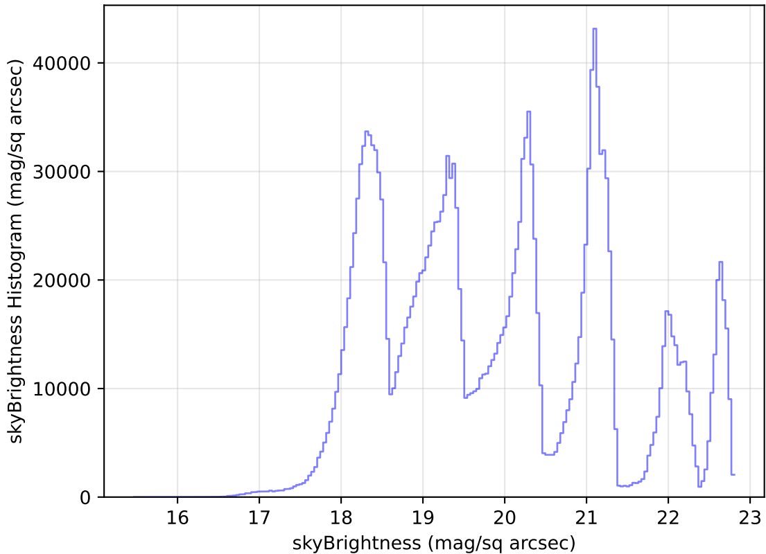
weather_cloudso1v3.4_10yrs WFD all bands: skyBrightness Histogram
