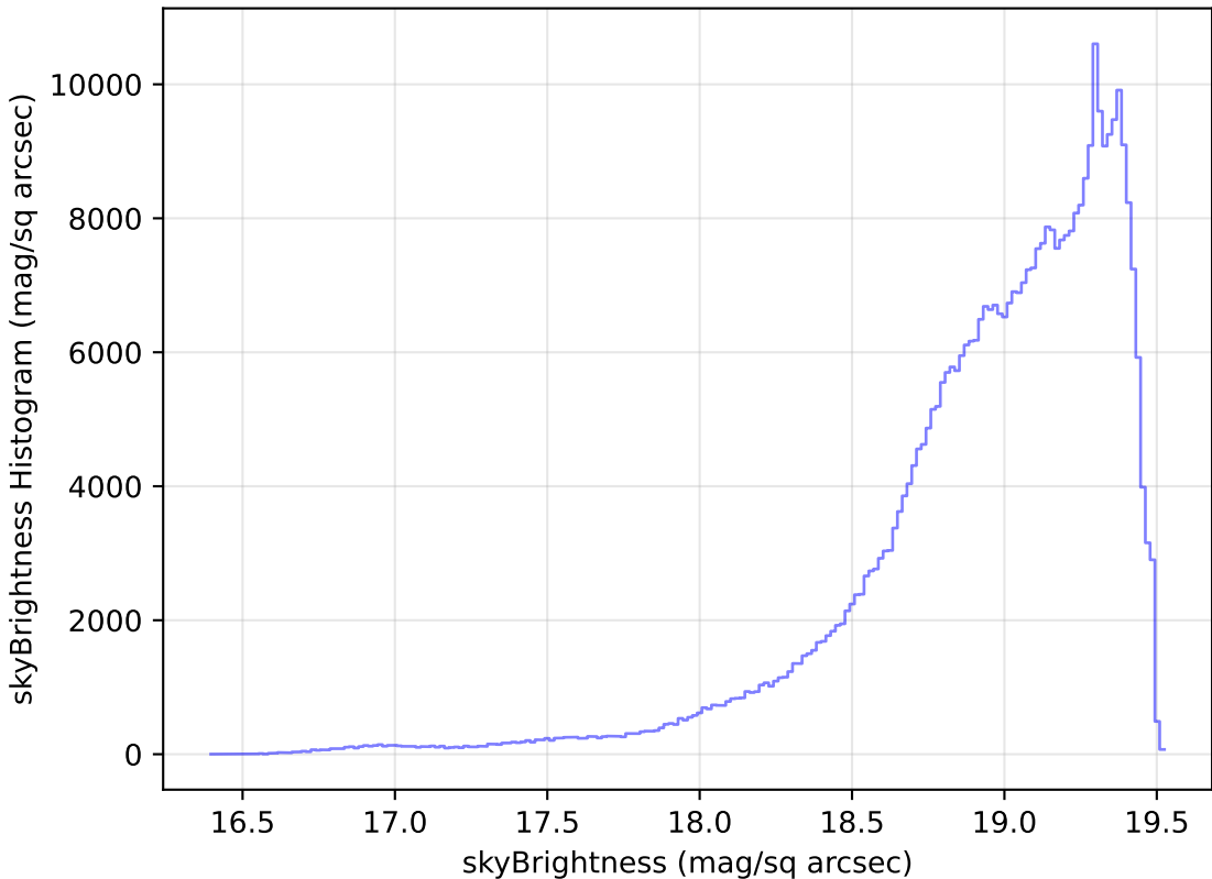
weather_cloudso1v3.4_10yrs All sky z band: skyBrightness Histogram
