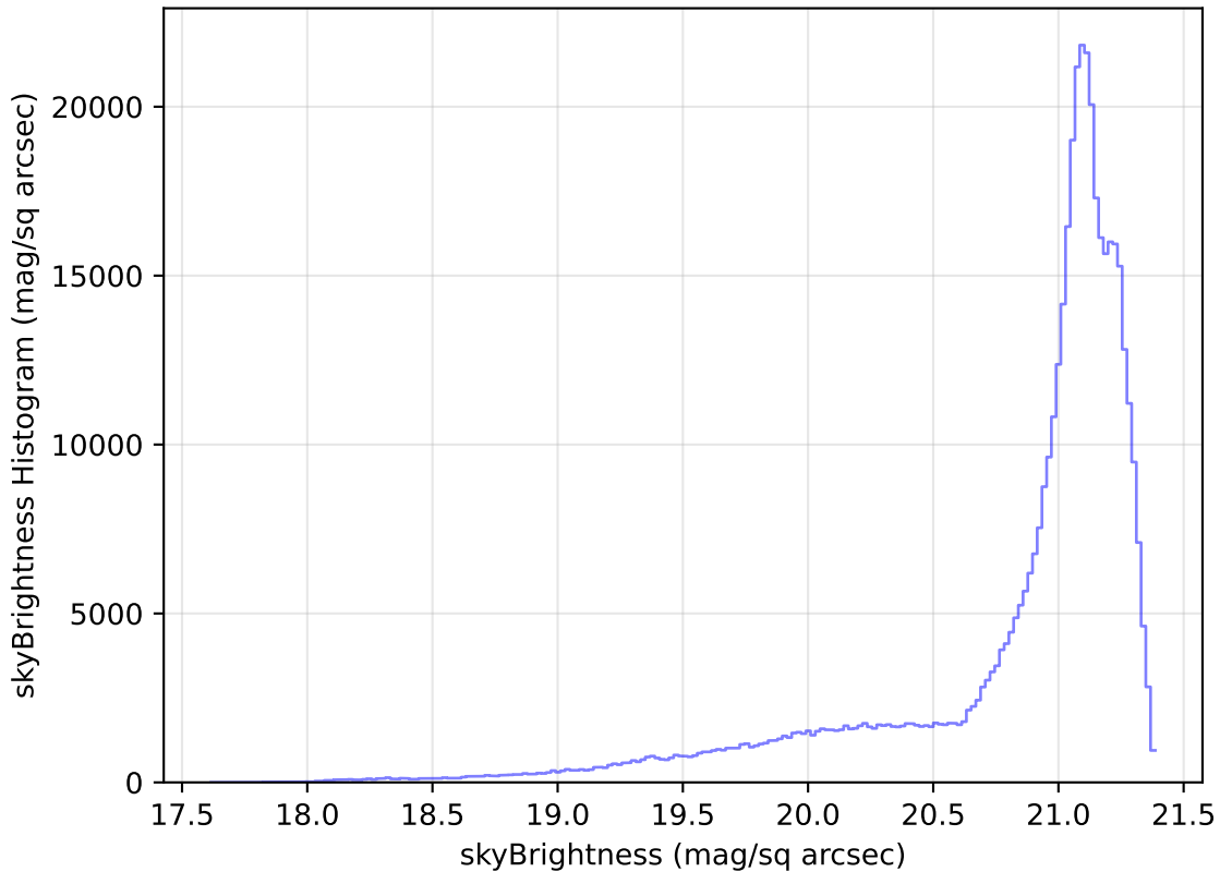
weather_cloudso1v3.4_10yrs All sky r band: skyBrightness Histogram
