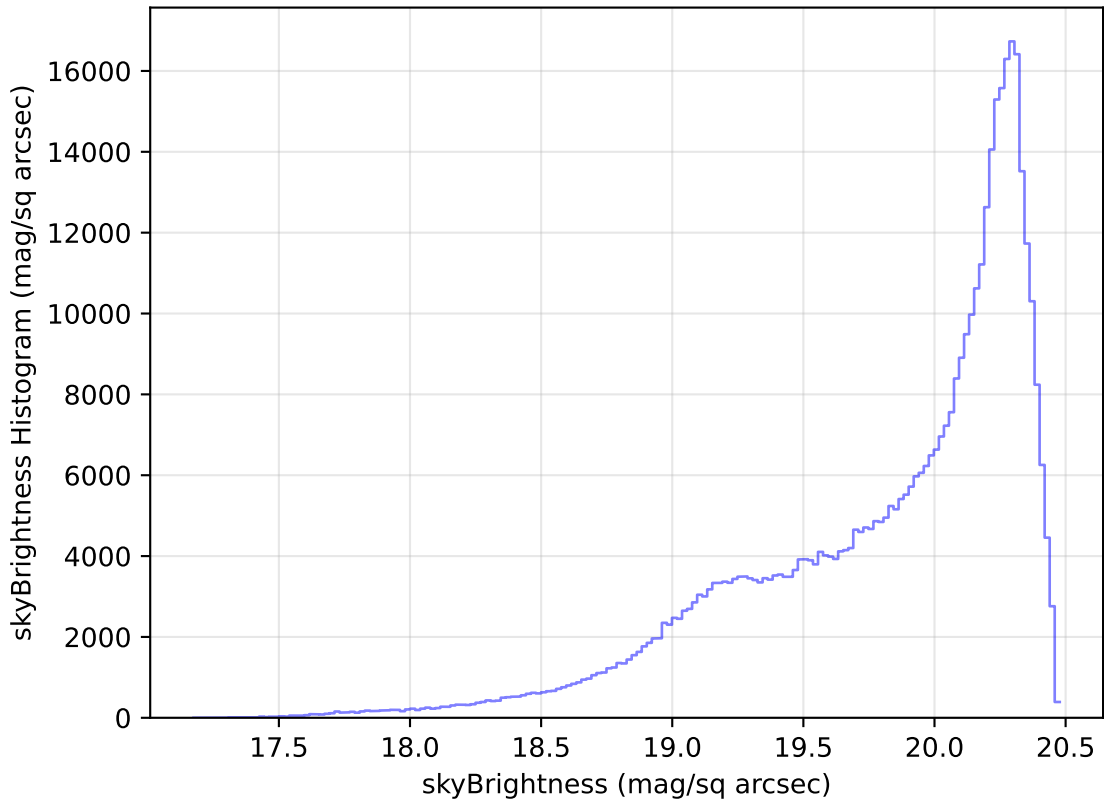
weather_cloudso1v3.4_10yrs All sky i band: skyBrightness Histogram
