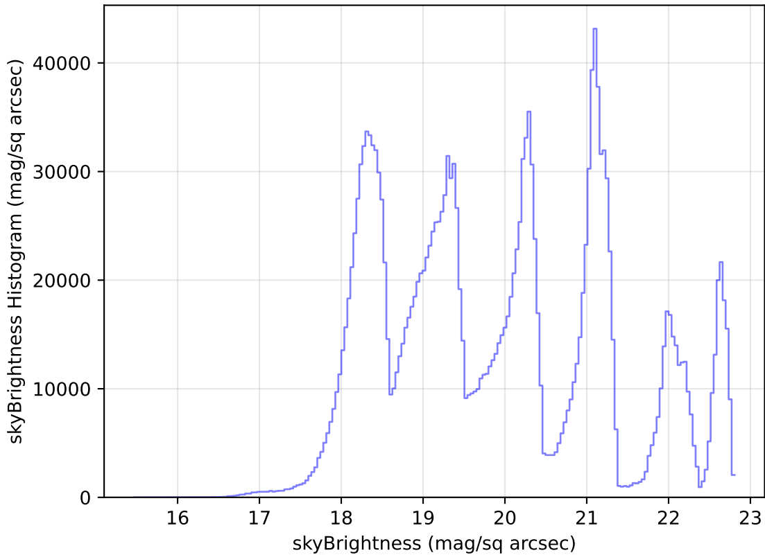
weather_cloudso1v3.4_10yrs All sky all bands: skyBrightness Histogram
