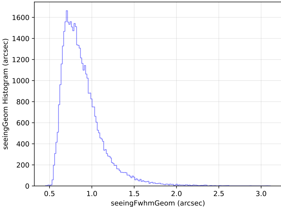
weather_cloudso1v3.4_10yrs Yr 1 z band: seeingGeom Histogram
