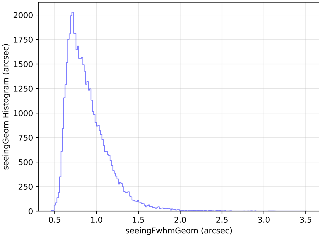
weather_cloudso1v3.4_10yrs Yr 1 r band: seeingGeom Histogram
