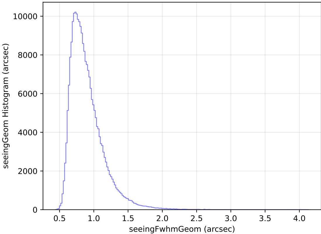
weather_cloudso1v3.4_10yrs Yr 1 all bands: seeingGeom Histogram
