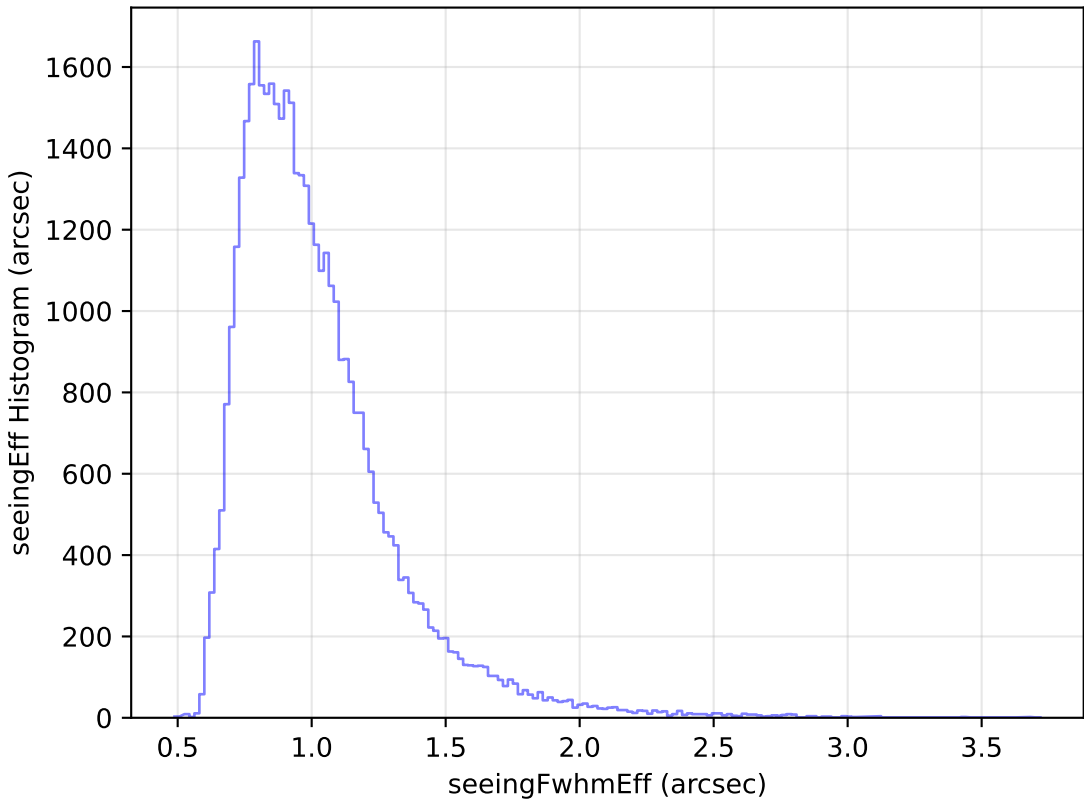
weather_cloudso1v3.4_10yrs Yr 1 z band: seeingEff Histogram
