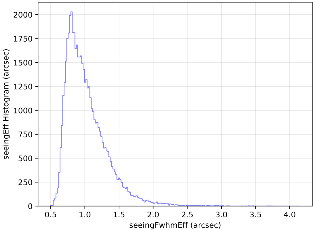
weather_cloudso1v3.4_10yrs Yr 1 r band: seeingEff Histogram
