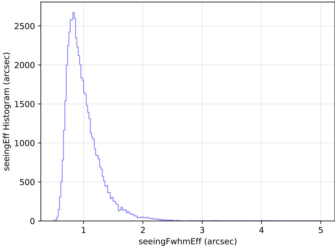
weather_cloudso1v3.4_10yrs Yr 1 i band: seeingEff Histogram
