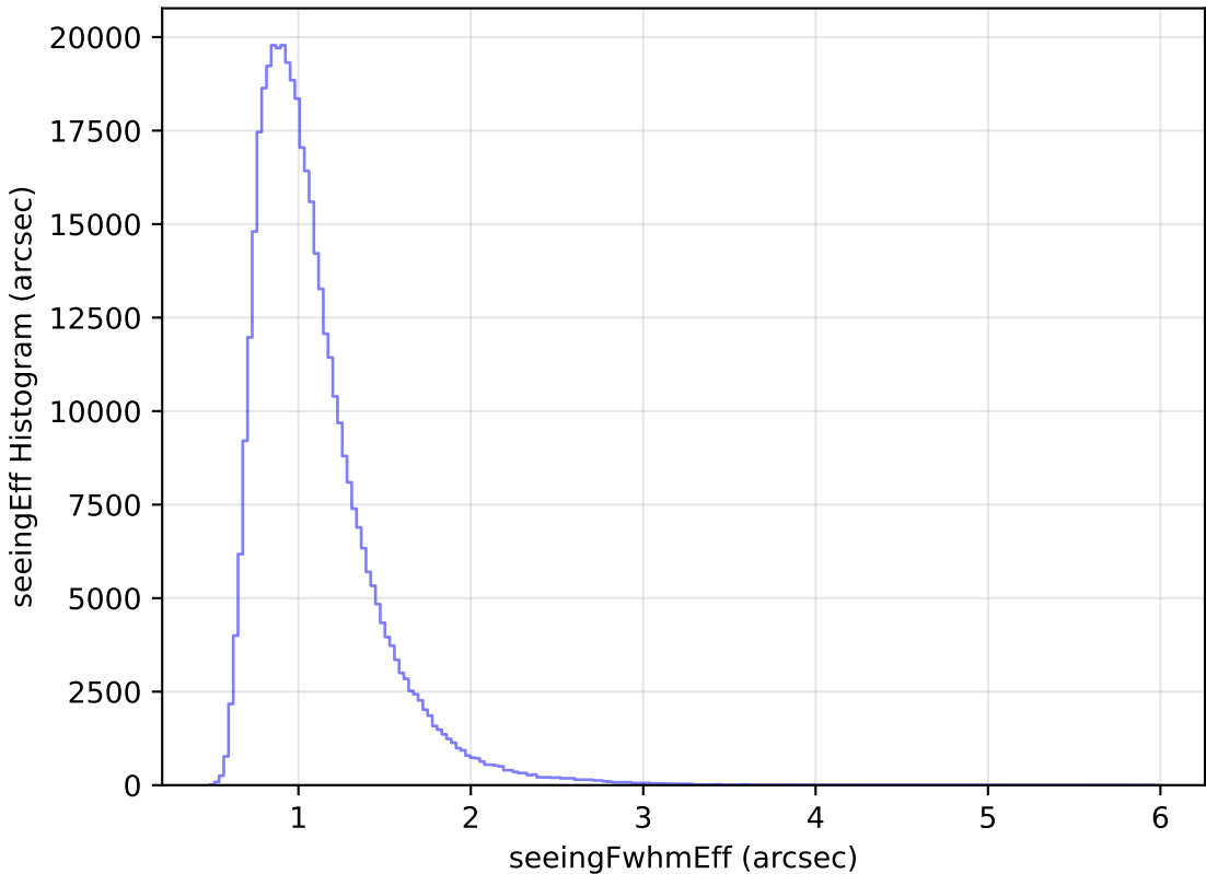
weather_cloudso1v3.4_10yrs WFD z band: seeingEff Histogram
