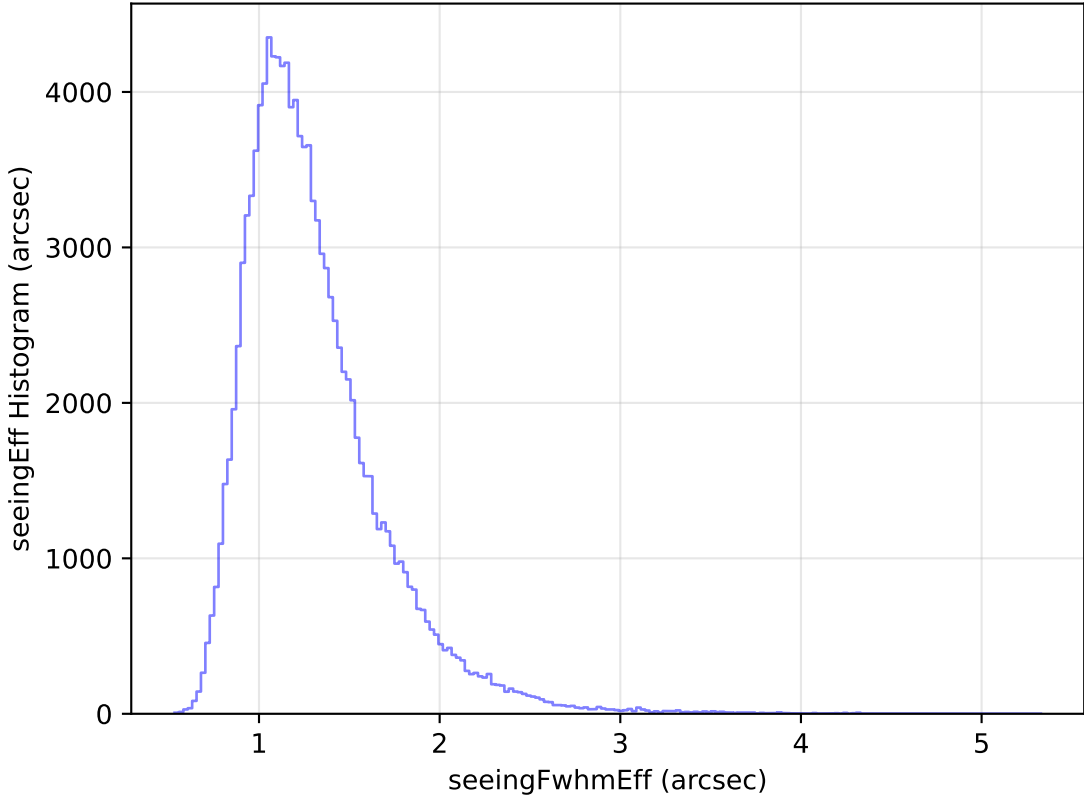
weather_cloudso1v3.4_10yrs WFD u band: seeingEff Histogram
