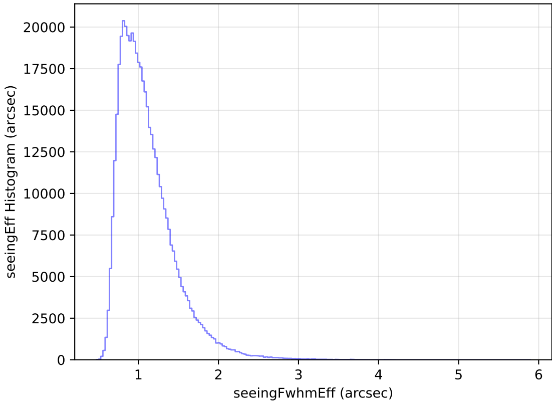
weather_cloudso1v3.4_10yrs WFD r band: seeingEff Histogram
