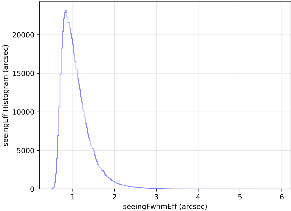
weather_cloudso1v3.4_10yrs WFD i band: seeingEff Histogram
