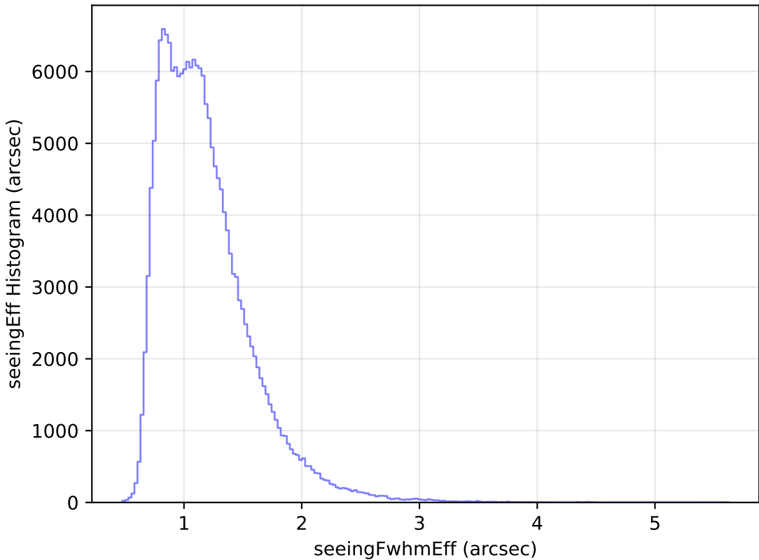
weather_cloudso1v3.4_10yrs WFD g band: seeingEff Histogram
