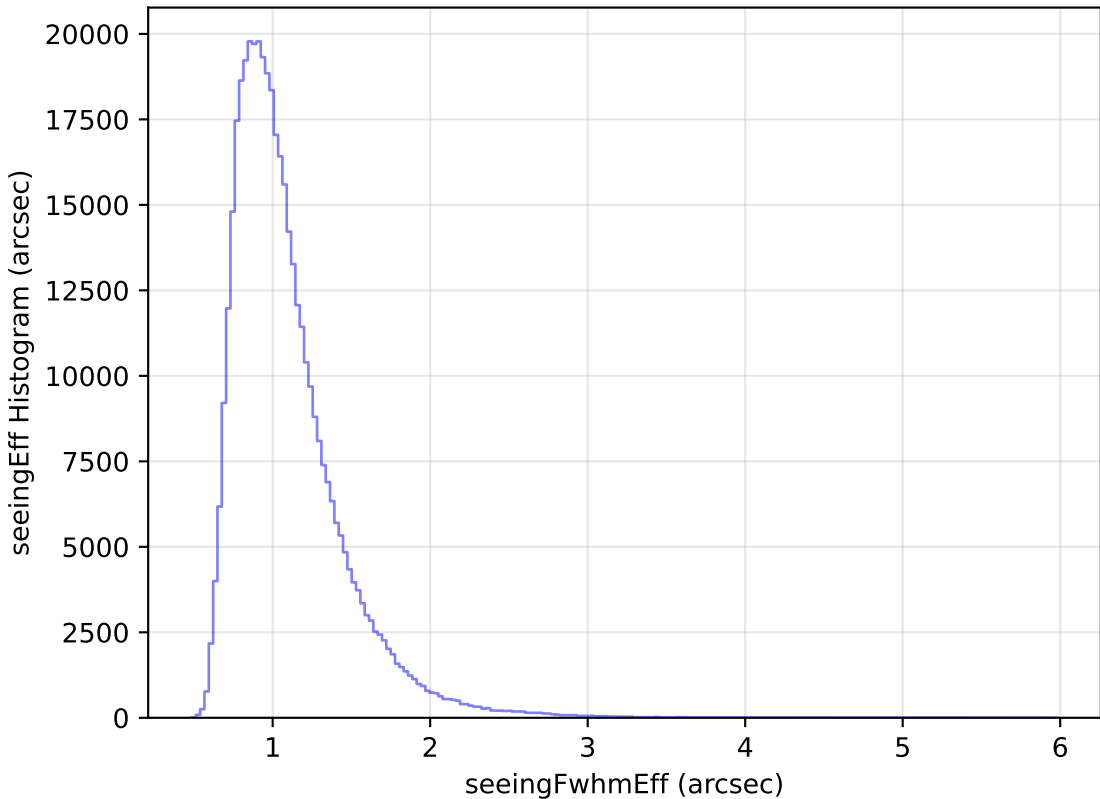
weather_cloudso1v3.4_10yrs All sky z band: seeingEff Histogram
