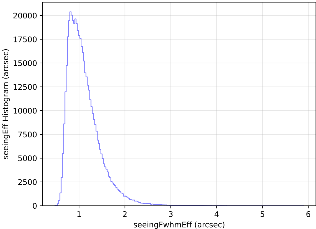
weather_cloudso1v3.4_10yrs All sky r band: seeingEff Histogram
