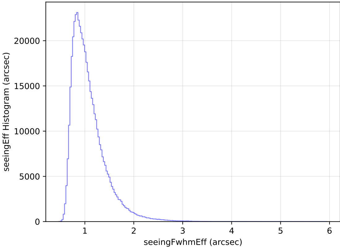
weather_cloudso1v3.4_10yrs All sky i band: seeingEff Histogram
