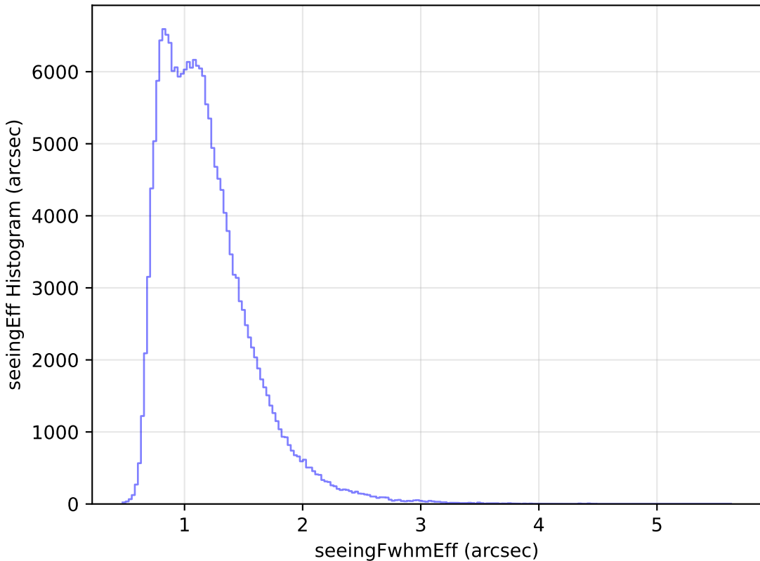
weather_cloudso1v3.4_10yrs All sky g band: seeingEff Histogram
