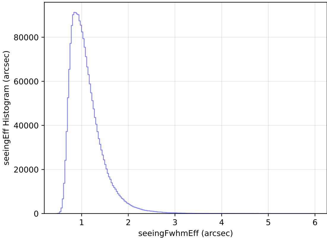
weather_cloudso1v3.4_10yrs All sky all bands: seeingEff Histogram
