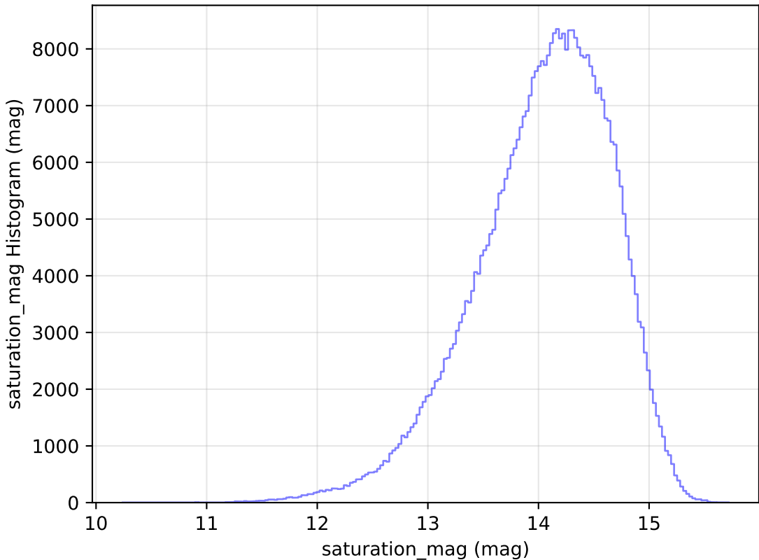
weather_cloudso1v3.4_10yrs WFD z band: saturation_mag Histogram
