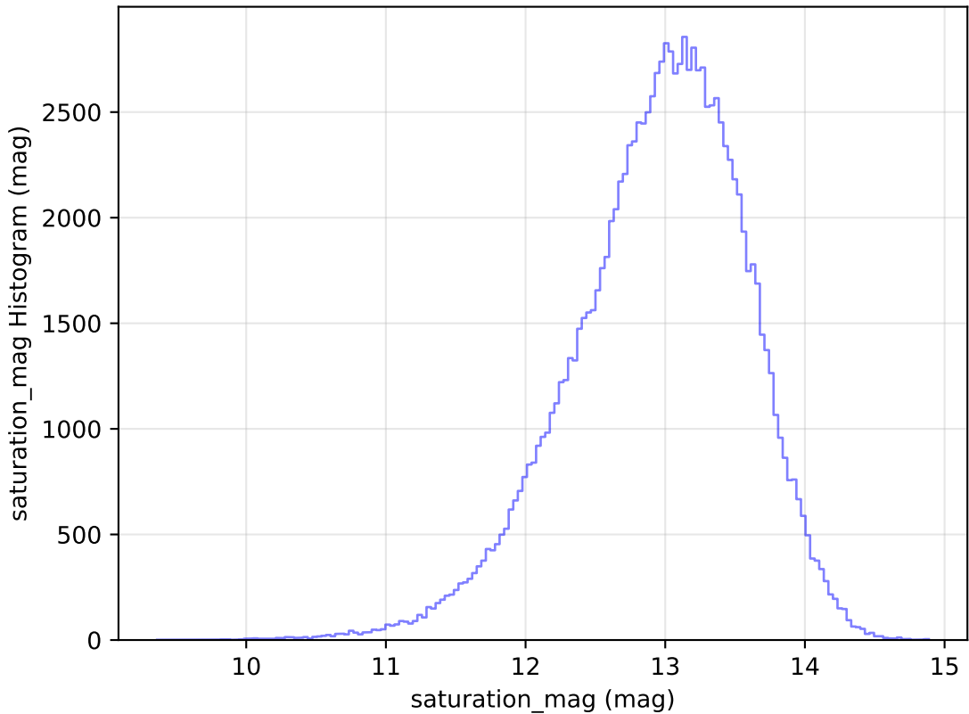
weather_cloudso1v3.4_10yrs WFD u band: saturation_mag Histogram
