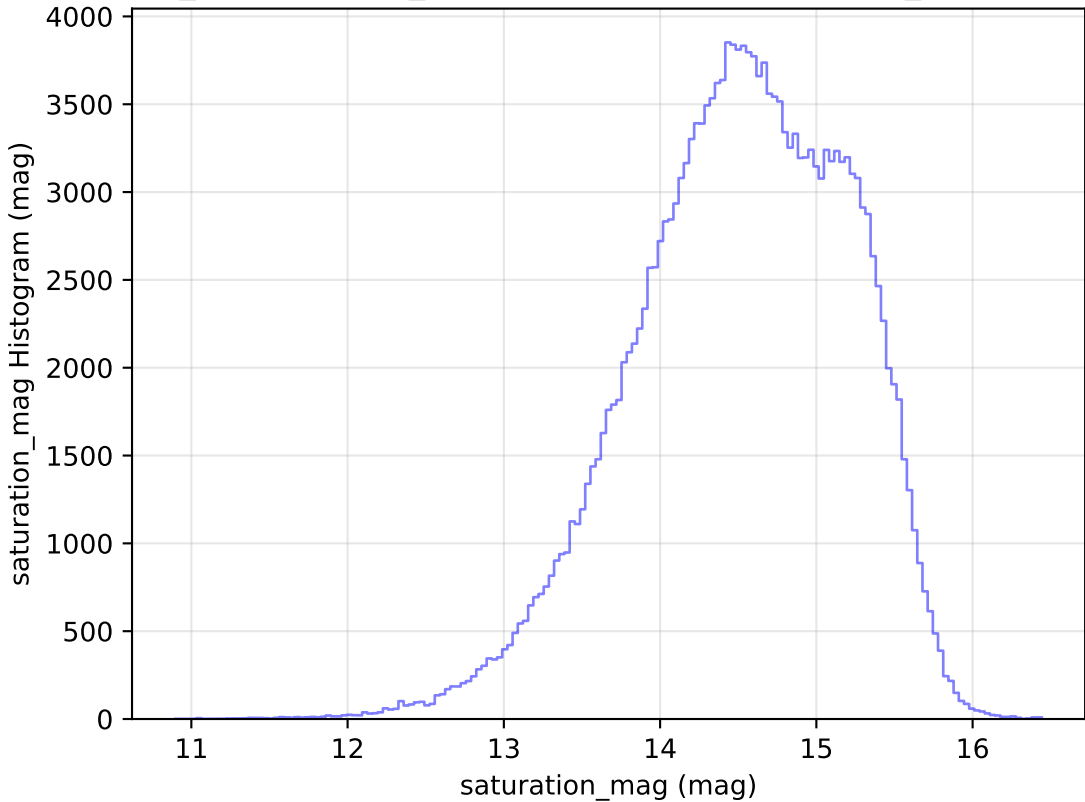
weather_cloudso1v3.4_10yrs WFD g band: saturation_mag Histogram
