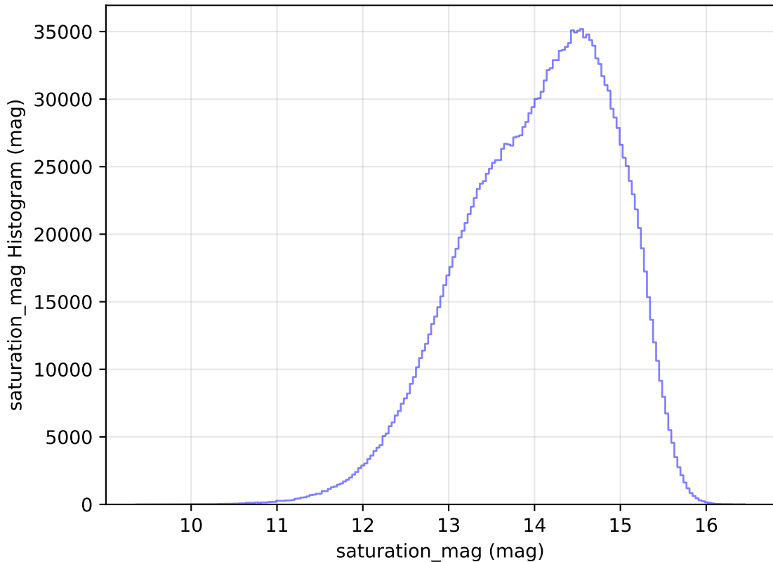
weather_cloudso1v3.4_10yrs WFD all bands: saturation_mag Histogram
