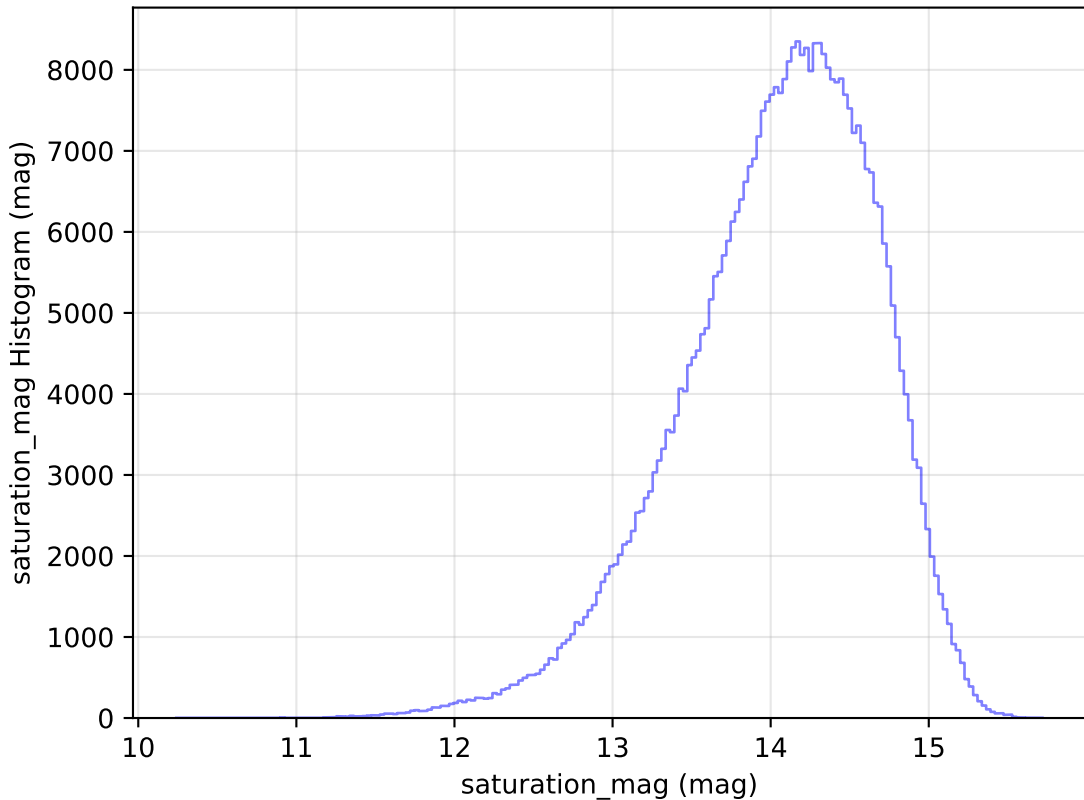
weather_cloudso1v3.4_10yrs All sky z band: saturation_mag Histogram
