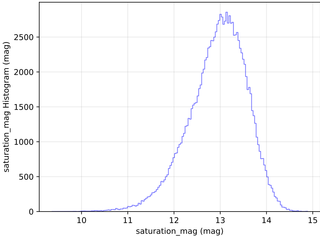
weather_cloudso1v3.4_10yrs All sky u band: saturation_mag Histogram
