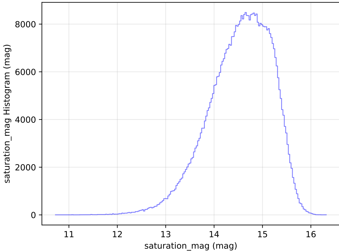
weather_cloudso1v3.4_10yrs All sky r band: saturation_mag Histogram
