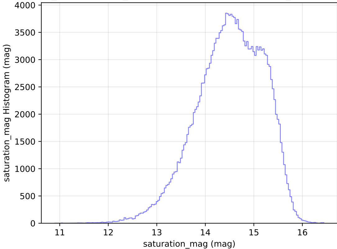
weather_cloudso1v3.4_10yrs All sky g band: saturation_mag Histogram
