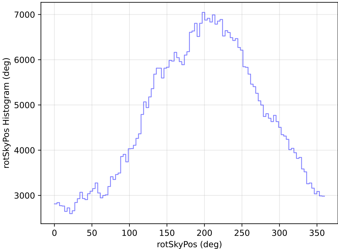
weather_cloudso1v3.4_10yrs WFD r band: rotSkyPos Histogram
