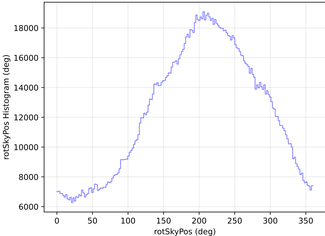
weather_cloudso1v3.4_10yrs WFD all bands: rotSkyPos Histogram
