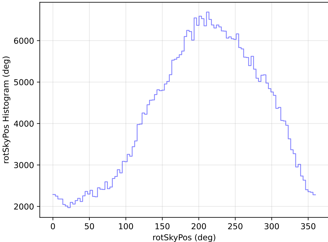
weather_cloudso1v3.4_10yrs All sky z band: rotSkyPos Histogram
